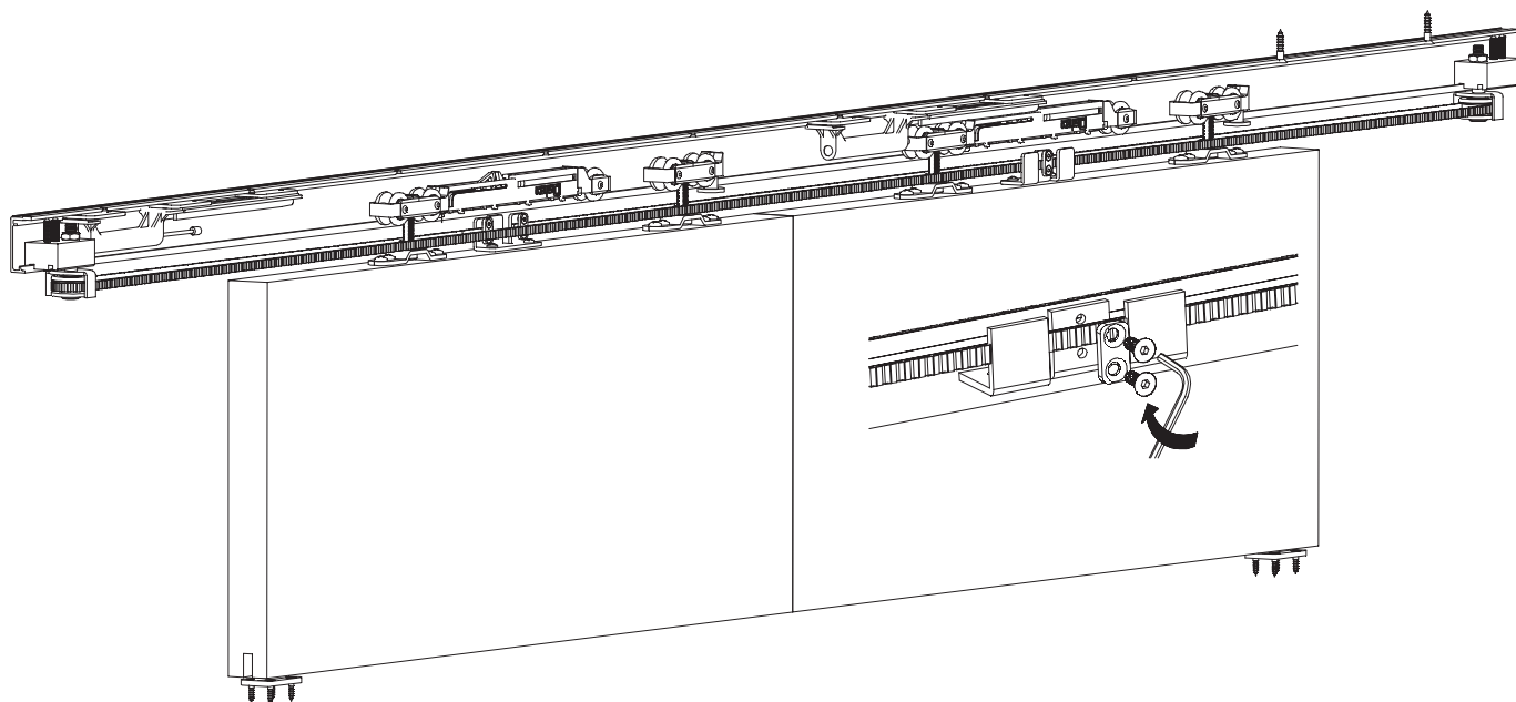
Synchronized system features an anti-jump feature attached to the rollers.
