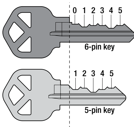
Figure 9. Comparing a 5-pin and 6-pin key
