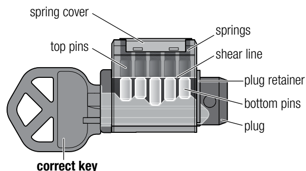
Figure 1. Correct Key Inserted
