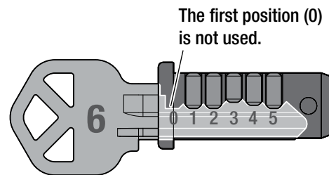
Figure 11. 6-pin key in 5-pin plug
