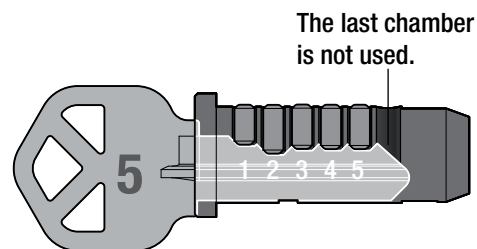
Figure 12. 5-pin key in 6-pin plug
