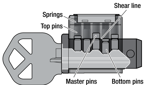
Figure 13. Master keyed Lock
