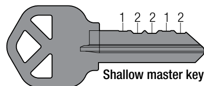
Figure 17. Deep and Shallow Master Keys
