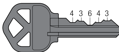
Figure 8. Key with a 4-3-6-4-3 Combination
