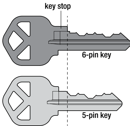
Figure 10. Longer key stop on a 6-pin key
