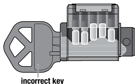
Figure 3. Incorrect Key Inserted
