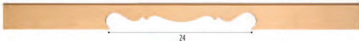
VAN- K2 60 x 4 1/2 x 3/4
