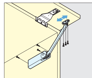
② Mount the OV-EZ mechanism to the side wall of the cabinet as illustrated in installation instructions provided with the product.
