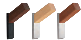
PREMIUM WOOD PXB-WM-5-111 Base: Zinc Alloy, Steel W22 x H96 x D64.5 (mm)
