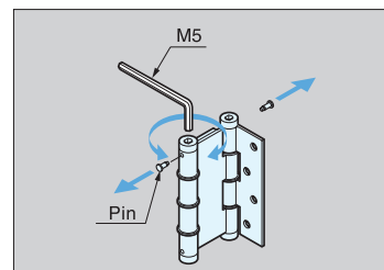
Spring Adjustment
