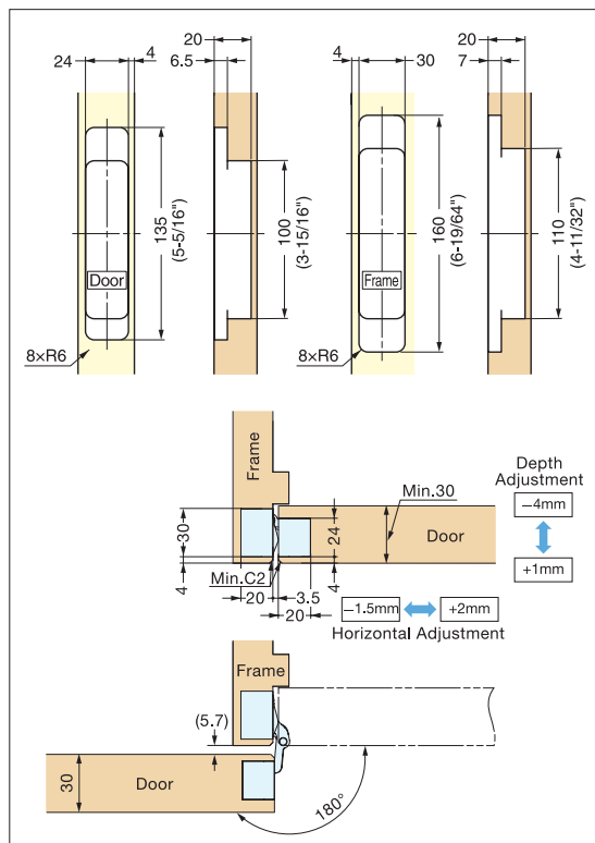
Bore Dimensions
