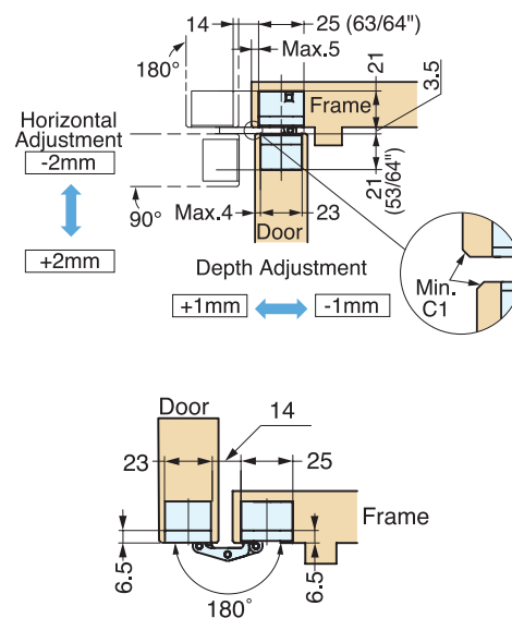
Bore Dimensions
