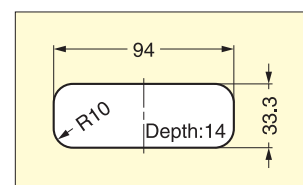
Cut out Dimensions
