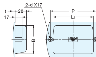
Handle Holding Fixture
