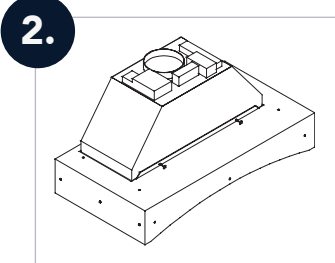
Assemble blower unit (sold separately) to metal liner
