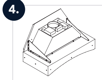
Hang the liner/bracket assembly on the mounting plate (make all electrical and ventilation connections at this point)
