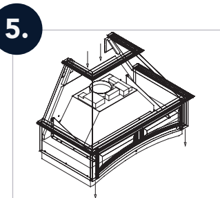
Slip the wood range hood on top of the mounting plate
