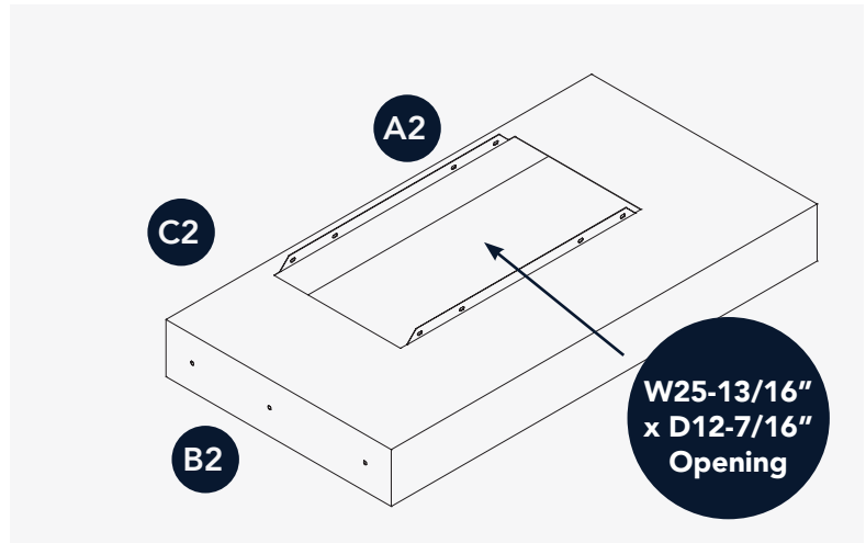
Liners Specifically Designed for Sirius 960CFM Ventilator
